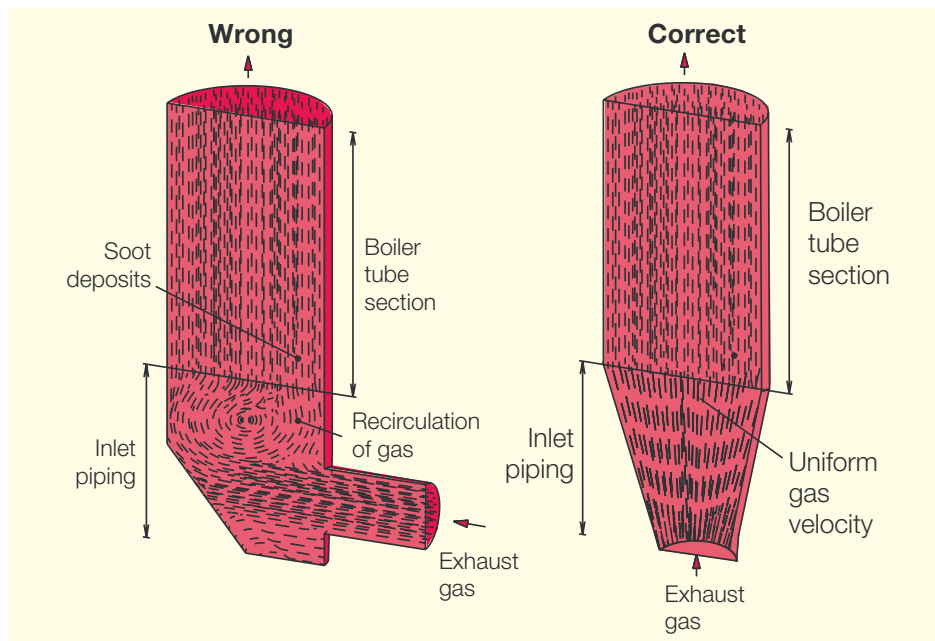
Fig. 22: Exhaust gas boiler – influence of inlet pipings
