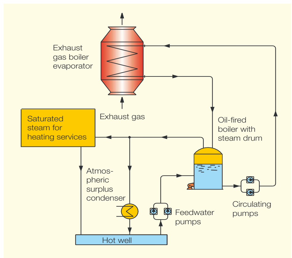
Fig. 7: Normal exhaust gas boiler system for steam production Single pressure steam system with evaporator section only
