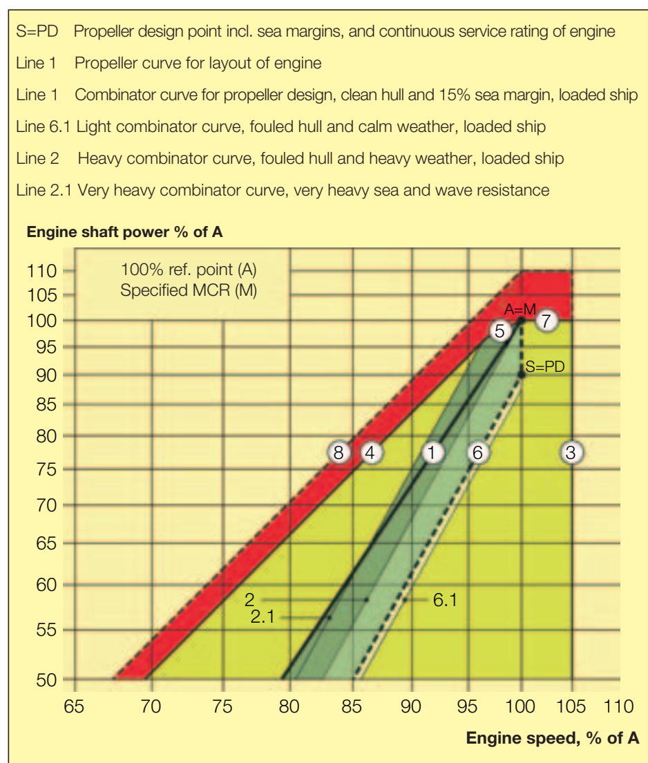
Fig. 25: Influence of ship resistance on combinator curves for CP-propeller
