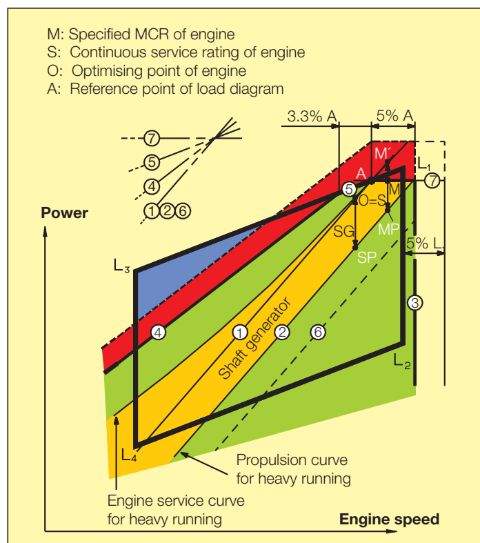
Fig. 22b: Example 4 with FPP – load diagram with SG (special case)
