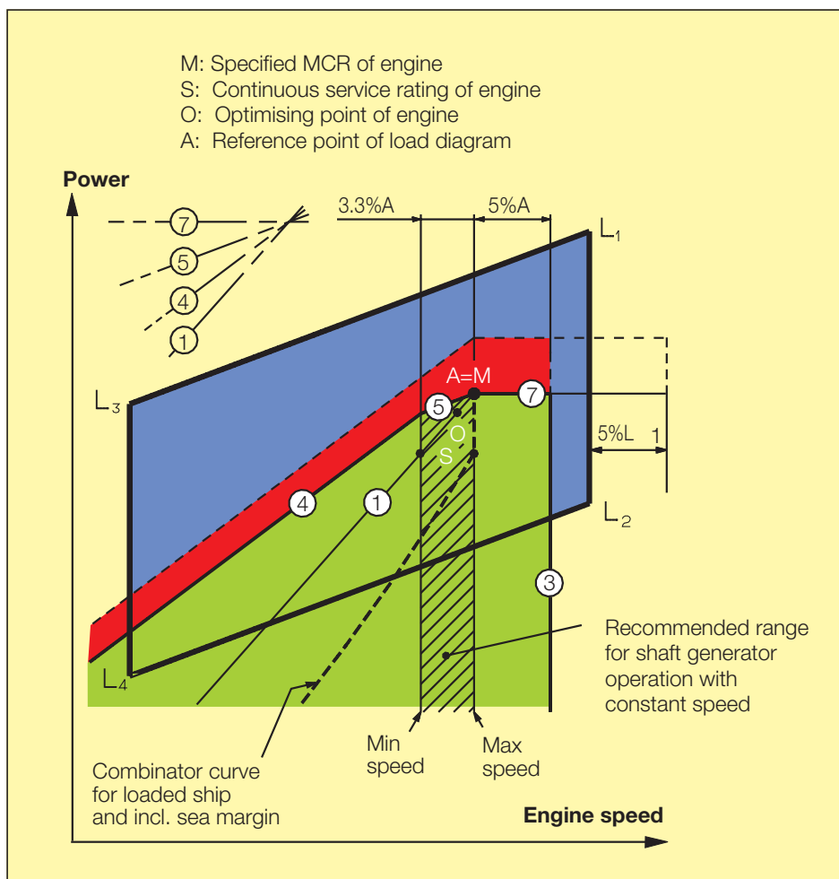
Fig. 23: Example 5 with CPP – with or without shaft generator
